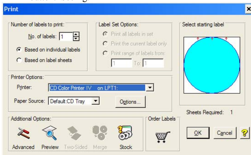
Fig.2 Print window.
